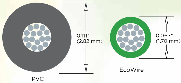
18 AWG (0.81) Wire
