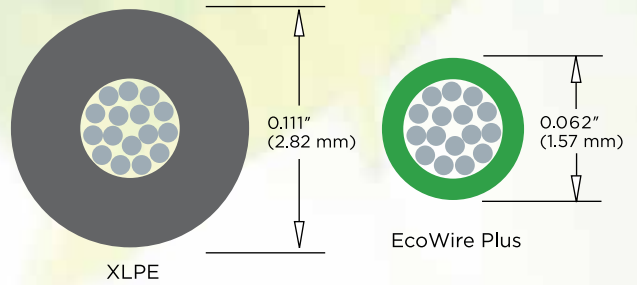
18 AWG (0.81) Wire
