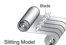
Slitting Model
